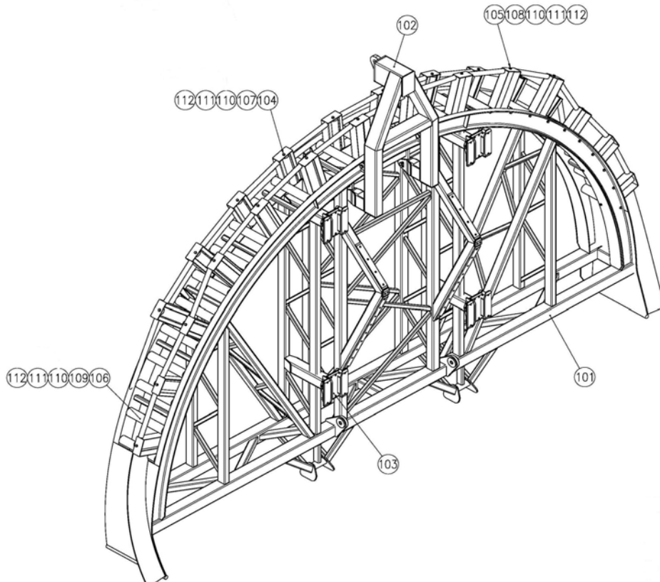
Cable Deployment Bow
